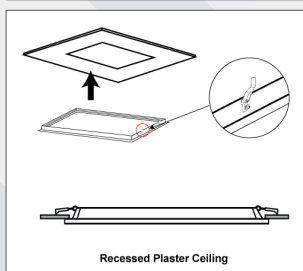
Recessed Plaster Ceiling
